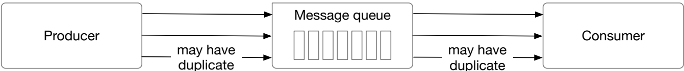
Figure 33 At-least once
