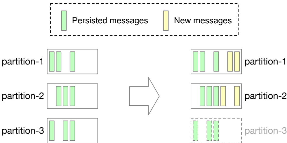
Figure 31 Partition decrease
