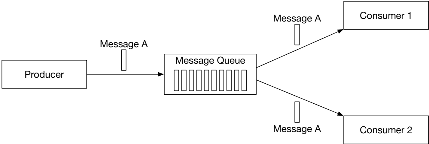
Figure 4 Publish-subscribe model
