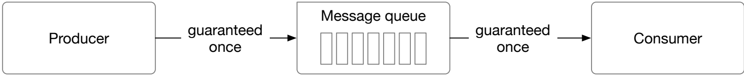
Figure 34 Exactly once
