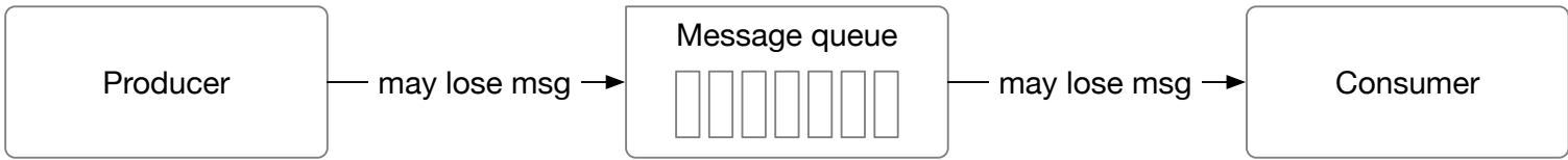
Figure 32 At-most once
