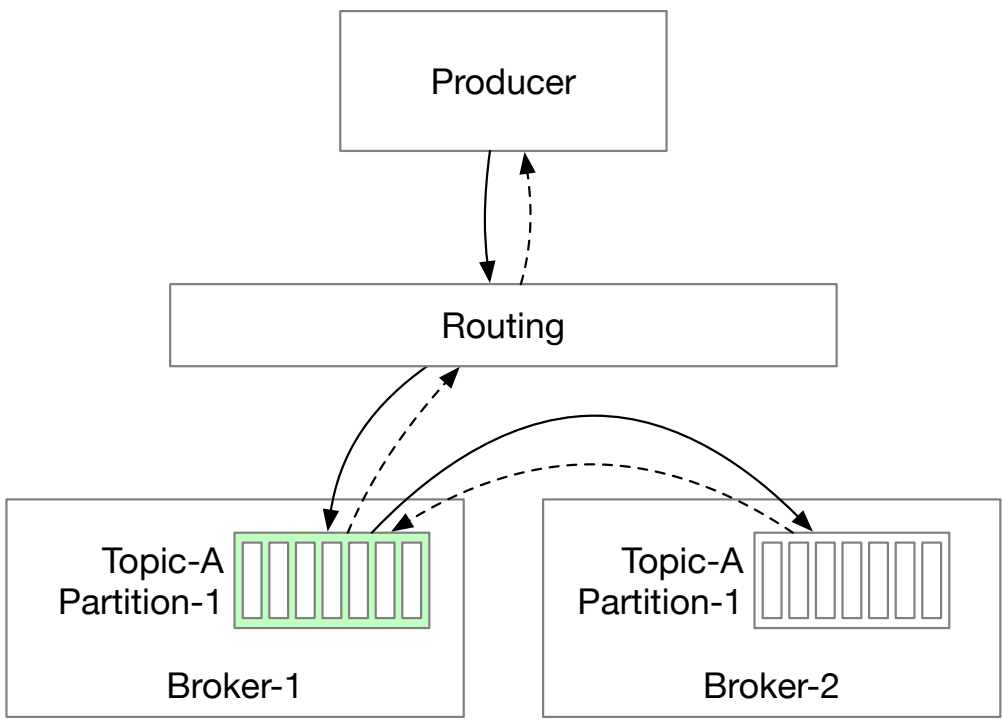
Figure 11 Routing layer
