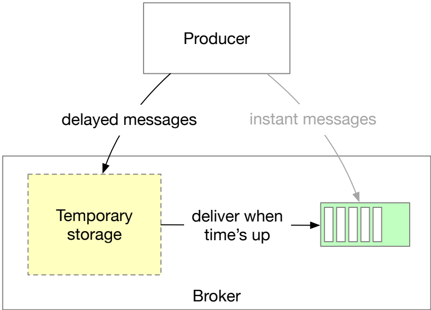
Figure 36 Delayed messages
