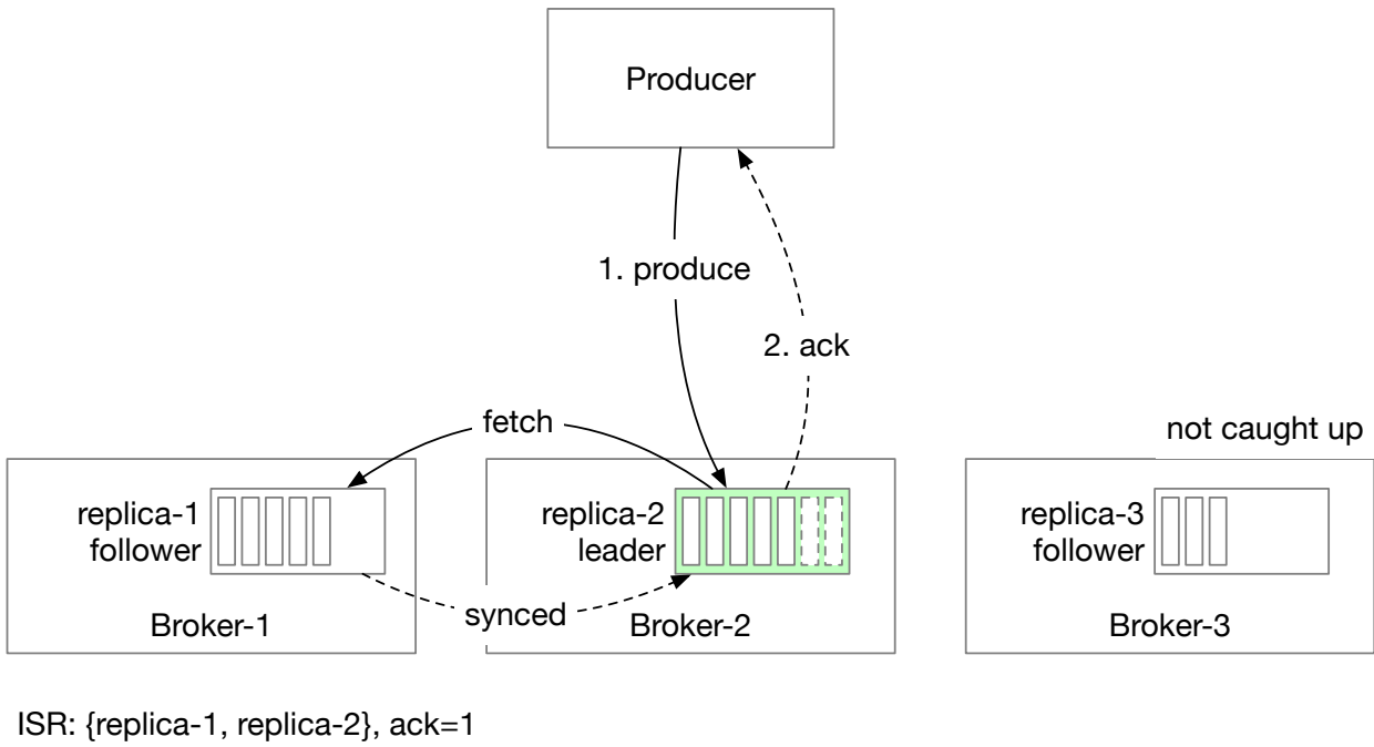
Figure 26 ack=1
