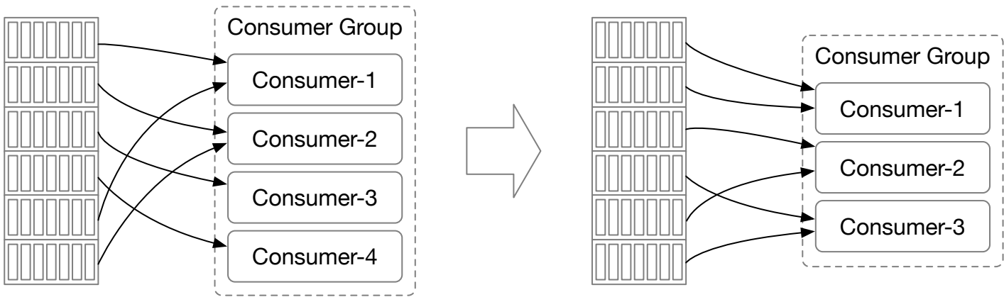
Figure 17 Consumer rebalance
