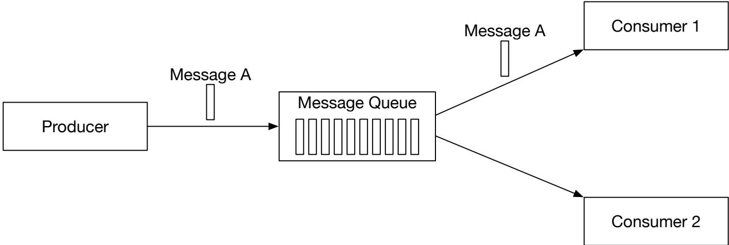
Figure 3 Point-to-point model
