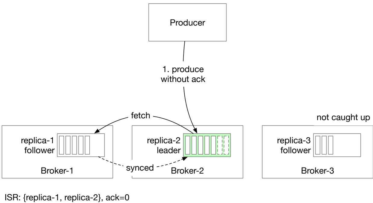
Figure 27 ack=0
