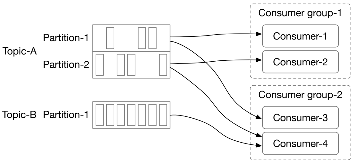
Figure 7 Consumer groups
