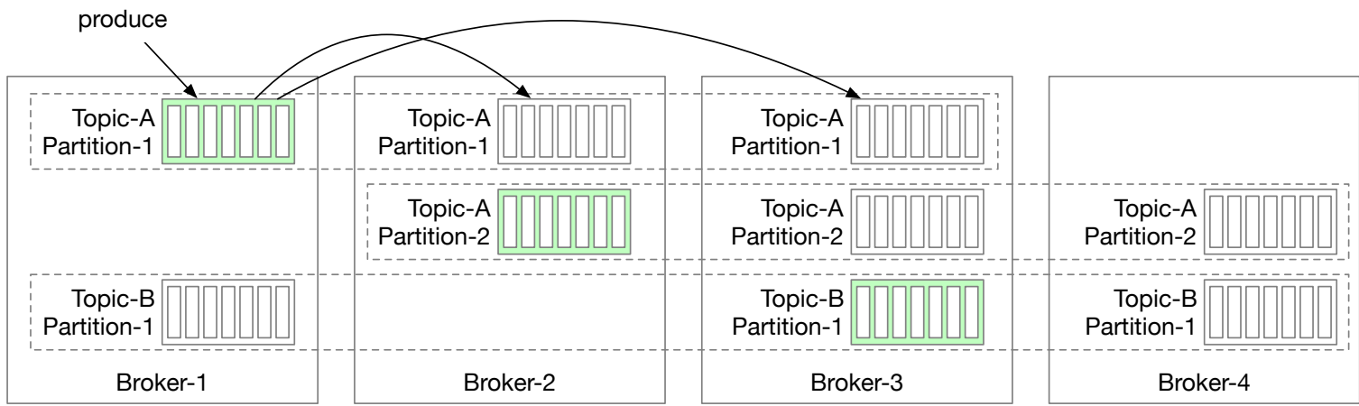
Figure 23 Replication
