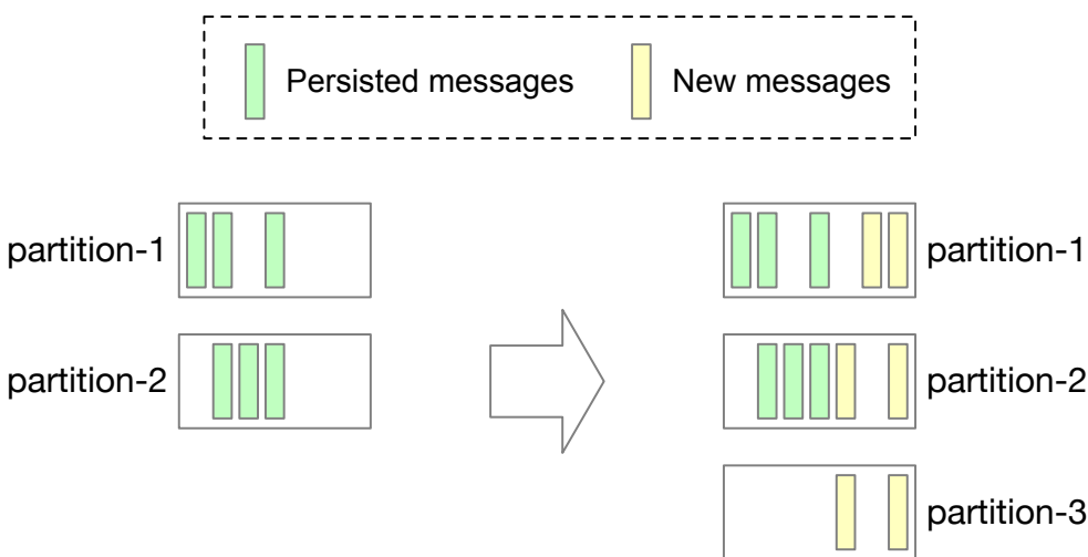
Figure 30 Partition increase
